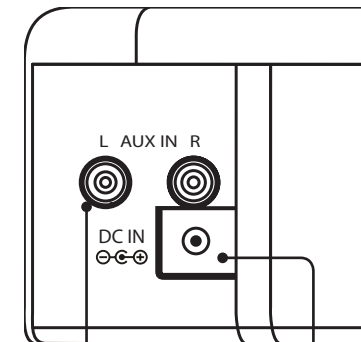
Aux In Requires RCA stereo audio cable (included). DC Power Port
